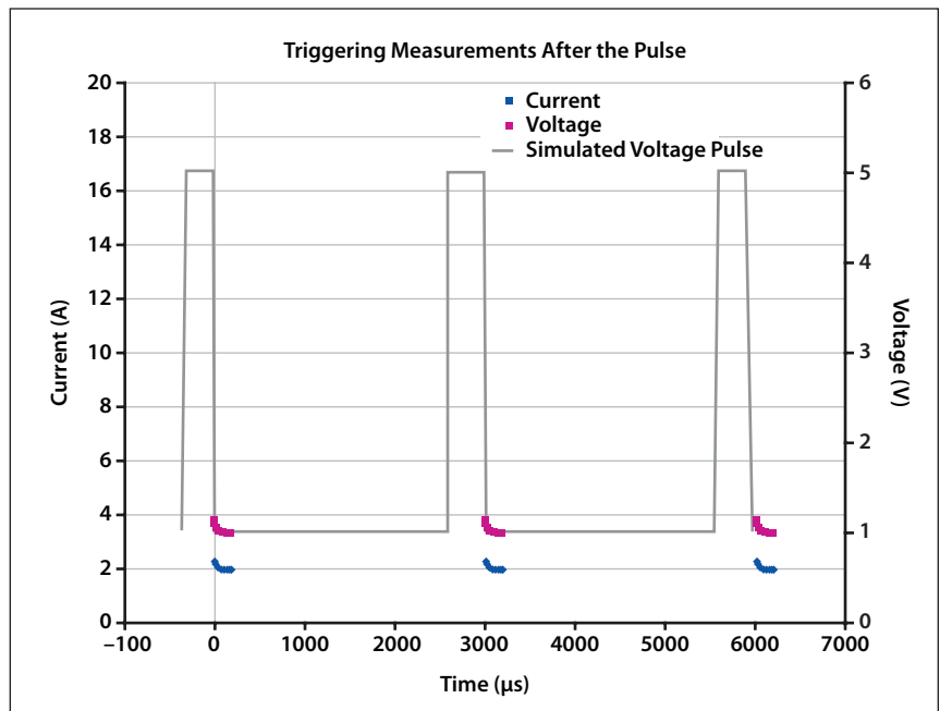
Figure 6: Results of post-pulse characterization. There is a 0.5Ω resistive load.
