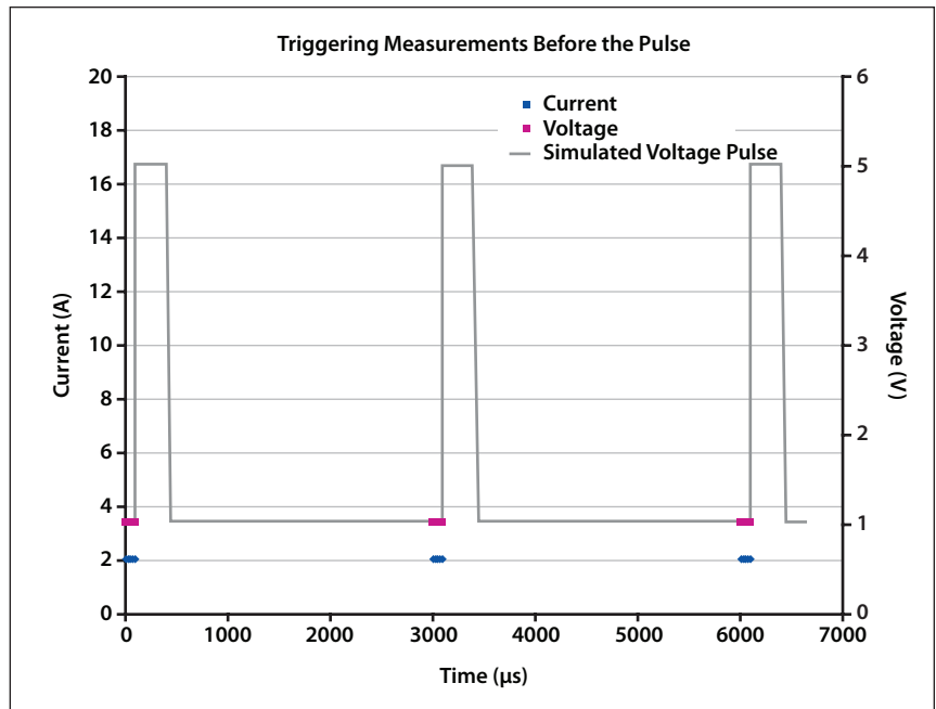
Figure 5: Results of pre-pulse characterization. There is a 0.5Ω resistive load.
