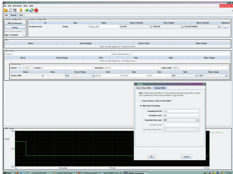
Figure 7: Use TSP Express software to configure pulses and perform measurements quickly with the high speed ADC.
